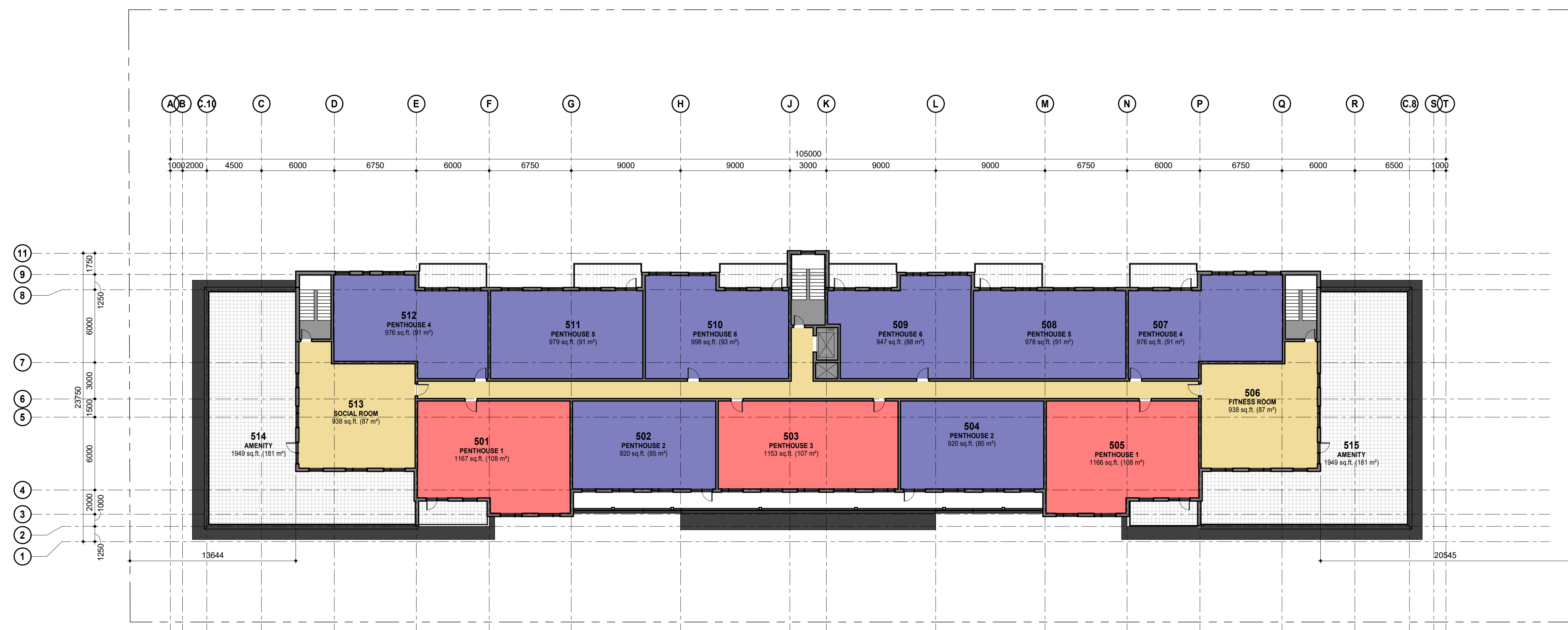
2 LEVEL 500 1:200
